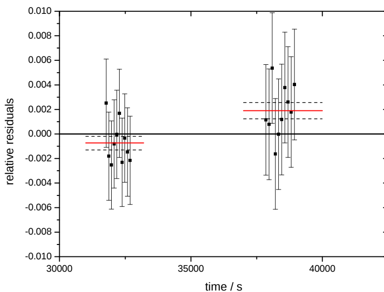
Figure 2. Example of relative residuals obtained for two series of measurements with the new SIR and a ^{99\text{m}}\text{Tc} ampoule at low current (radius source 1). The red lines and dotted lines correspond to the mean relative residuals and the standard deviation of the mean. On the left no significant ( k = 2 ) deviation from zero is observed. On the right the residuals are systematically above zero.
